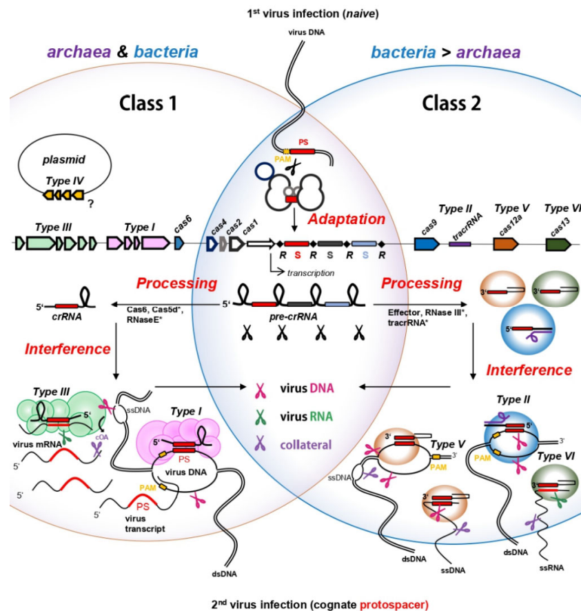
Figure 1. CRISPR types in prokaryotes and their mechanisms of action. Class 1 systems (including types I, III, and IV) are prevalent in both archaea and bacteria, whereas Class 2 systems (including types II, V and VI) are found almost exclusively in bacteria. Mechanisms and genes in the overlapping region are shared by the two classes. The different CRISPR steps are indicated in red and explained in the main text. Both classes contain effector complexes that can perform all three types of interference: virus DNA interference (indicated by pink scissors), virus RNA interference (indicated by green scissors) and collateral damage (i.e., promiscuous cleavage of host and virus DNA/RNA, indicated by purple scissors). “S” refers to “spacer”, “R” refers to “repeat”. * Asterisks refer to enzymes that are not involved in processing of all classes: Cas5d replaces Cas6 function in type I-C [25]; RNaseE is involved in processing in a type III-B system [26]; RNase III processes pre-crRNA in type II; tracrRNA is needed in type II and certain subtypes of type V (see text). Type I-D targets ssDNA and dsDNA (not shown) [27]; In type II systems, Csn2 is also involved in spacer acquisition (not
