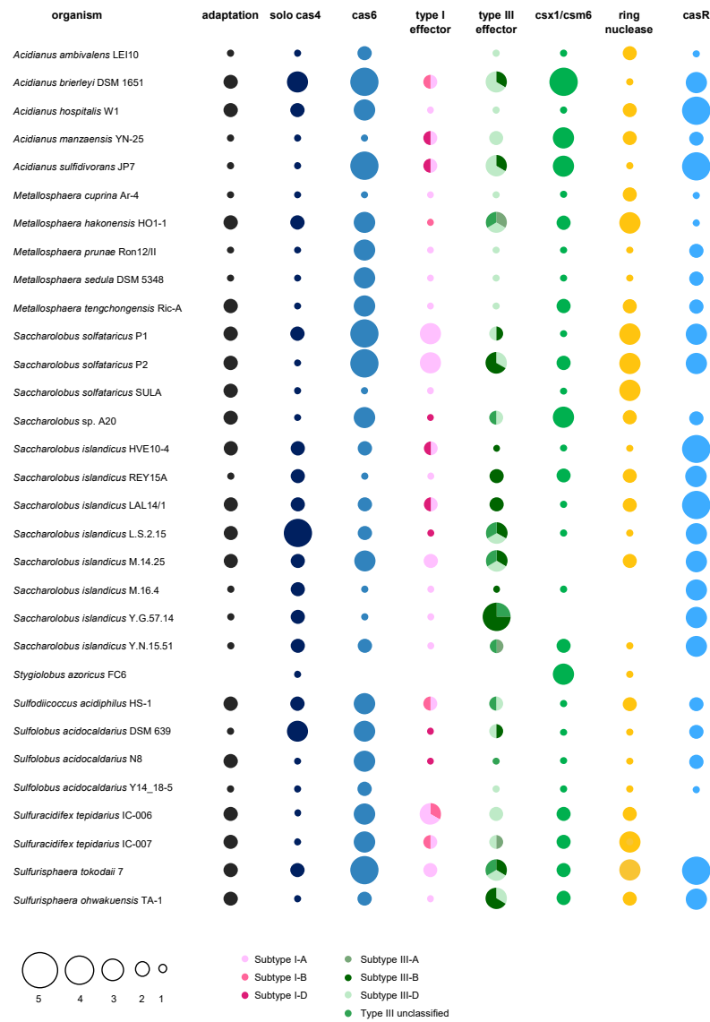
Figure 4. Distribution of CRISPR-Cas (sub)types and accessory genes in Sulfolobales genomes. The bubble plot shows the distribution and abundance of genes encoding proteins and protein complexes partaking in the CRISPR-Cas immune response in Sulfolobales genomes. The abundances of adaptation cassettes ( cas1-cas2 , frequently also cas4 ), cas6 (crRNA processing) and CRISPR-Cas effectors (interference) are depicted by size; abundances of the different subtypes of CRISPR-Cas effectors are indicated by different color shadings. Some adaptation cassettes contain either a cas1 or cas2 gene with internal stop codon or frameshift, highlighted in Supplementary Table S1. Additionally, abundances of solo cas4 (not encoded within 15 ORFs with respect to other adaptation genes) and accessory genes csx1/csm6 , crn (ring nuclease), casR (specific transcriptional regulator) are illustrated by bubbles in corresponding sizes. In cases with great overlap between different strains of the same species, only one genome is shown as a representative for all similar strains (e.g., S. solfataricus SULA and derivative strains). The analysis is based on data published in [19], and/or obtained by using programs CRISPRminer (version 1, [258]), CRISPRCasFinder (version CRISPR-Cas++ 1.1.2, [241]), and BLAST ([262,263]); BLAST analysis of Crn and Csx1 was performed based on amino acid sequences of the respective biochemically and structurally characterized proteins [139,144].
