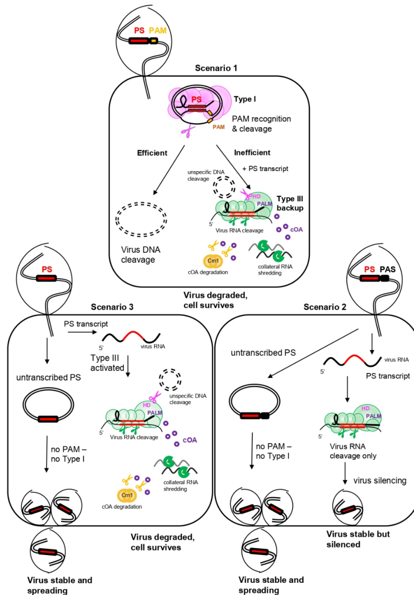
Figure 6. Three scenarios of anti-virus immunity in a Sulfolobales cell. Scenario 1 (PAM) would be the most efficient to degrade a virus in a Sulfolobales cell, whereas scenario 3 (no PAM, no PAS) could lead to virus spreading and/or cell death. Scenario 2 (PAS) is the only scenario that could lead to virus silencing on RNA level and, consequently, persistence of the virus in the population.
