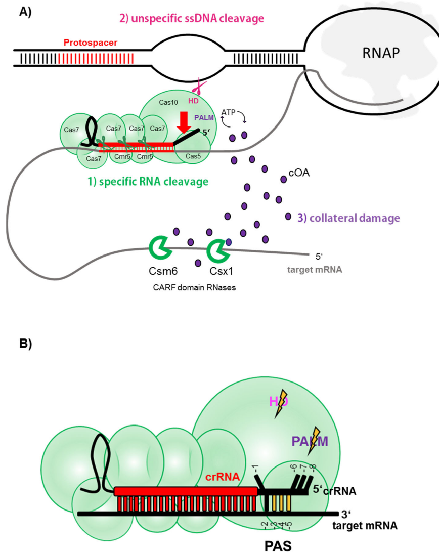
Figure 2. Activated and deactivated immune response of CRISPR type III complex. (A) The three phases of type III-mediated immunity are activated when a nascent mRNA is recognized by a crRNA in a type III complex. (1) Specific RNA cleavage: The Cas7 backbone cleaves the mRNA specifically at the protospacer region. (2) Unspecific ssDNA cleavage: When crRNA 5' handle and PAS are unpaired (red arrow), the HD domain (pink) of the large subunit Cas10 is activated and mediates sequence-unspecific ssDNA cleavage of nearby DNA bubbles. (3) Collateral RNA shredding: As in the case for ssDNA activation, the PALM domain (violet) in the large subunit Cas10 is activated if the 5' handle is unpaired to the PAS (red arrow). The PALM domain converts ATP into cyclic oligoadenylates which bind to the CARF domain of RNases, such as Csm6 and Csx1, thereby activating nonspecific RNA shredding. (B) Base pairing between the 5' handle of the crRNA and the 3' PAS. Complementarity in regions -3, -4, -5 deactivates HD and PALM domain activity, thereby only allowing specific RNA cleavage mediated by the backbone of the complex. Nucleotides in position -1, -6, -7, -8 do not contribute to base pairing, as they are distorted (-1), or tightly bound into specific pockets (-6, -7, -8).
