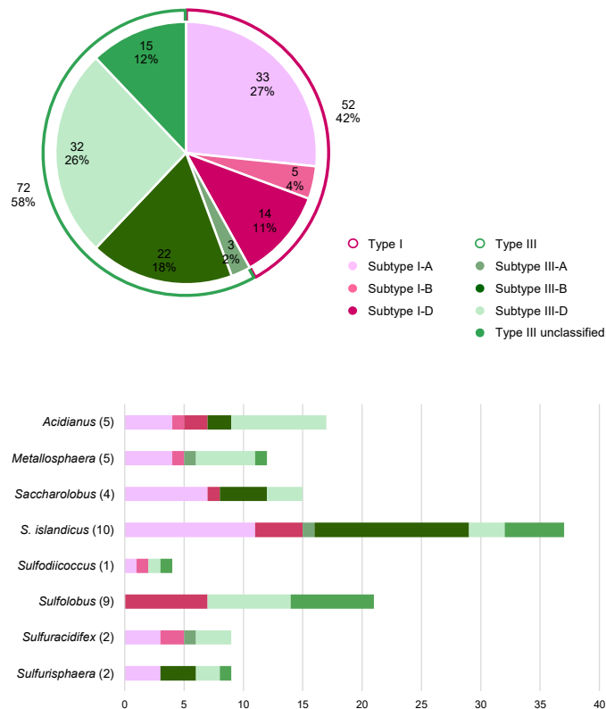
Figure 3. Presence of specific CRISPR-Cas (sub)types and their abundances among Sulfolobales genera. Overall abundances of CRISPR-Cas types and the specific subtypes within the general types I and III found in the order Sulfolobales (Upper panel). The bar chart shows the distribution of the CRISPR-Cas subtypes throughout the genera within Sulfolobales (Lower panel). The number of genomes included in the analysis for each genus is given in brackets. The analysis is based on data published in ref. [19] and/or obtained by using programs CRISPRminer (version 1, [258]), and CRISPRCasFinder (version CRISPR-Cas++ 1.1.2, [241]).
