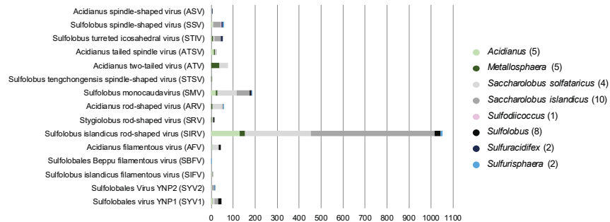
Figure 5. CRISPR array, spacers and virus matches in Sulfolobales genera. (A) The number of arrays (depicted in different color shadings) and the number of spacers per array are shown for representative genomes of the Sulfolobales. (B) The stacked bar plot shows the total amount of spacers identified on the genus level that (partially) match protospacers carried on genomes of viruses associated with the Sulfolobales. The data (CRISPR arrays and spacer) for the analyses were retrieved using programs CRISPRCasFinder (CRISPR-Cas++ 1.1.2, [241]) and orientation of CRISPR arrays was determined using CRISPRstrand (implemented in CRISPRmap v1.3.0-2013, [265,266]). Virus matches were identified using BLAST+ (version 2.10.0, [267]), spacers were blasted against the NCBI viral genomic RefSeq database [268] specifying the following parameters: word size = 8, e-value ≤ 0.01. Results were filtered for a query coverage ≥ 85% (calculated by dividing the alignment length by the query length) and allowing for a maximum number of 5 mismatches (see Supplementary Table S1), duplicate hits of a spacer to the same virus were removed.
